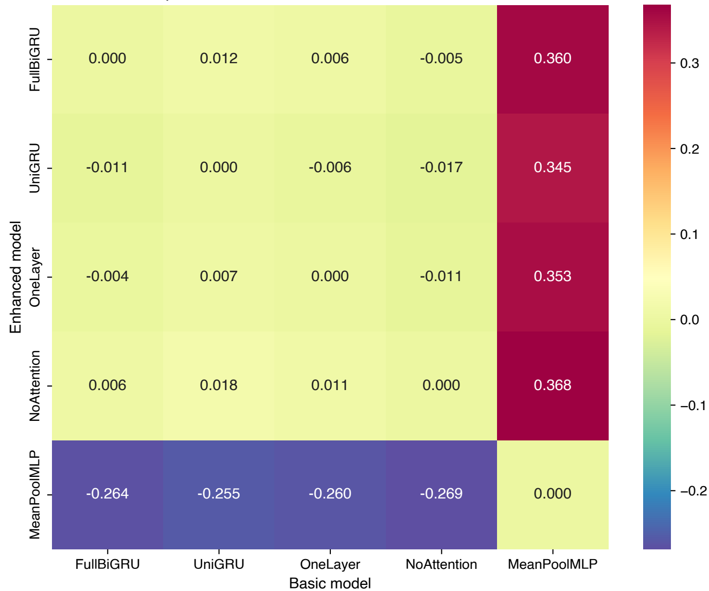
UCI HAR upstairs/downstairs directional IMV, mean of 10 seeds
