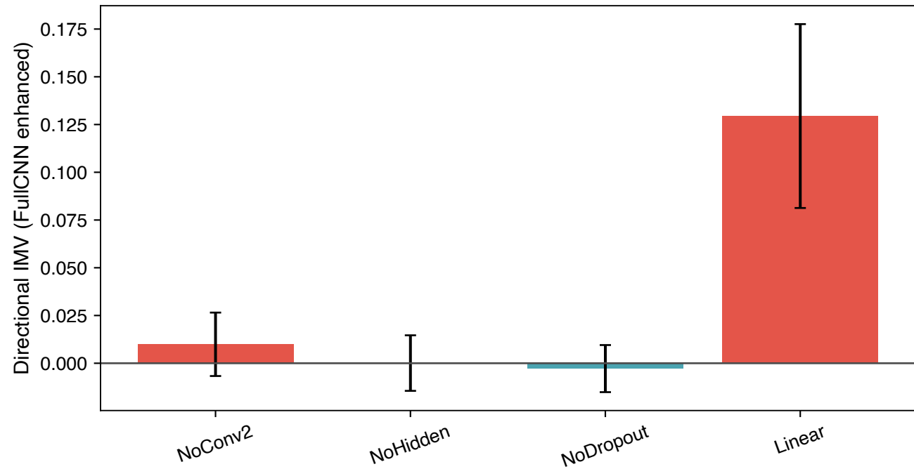
Full MNIST CNN relative to each ablated model
