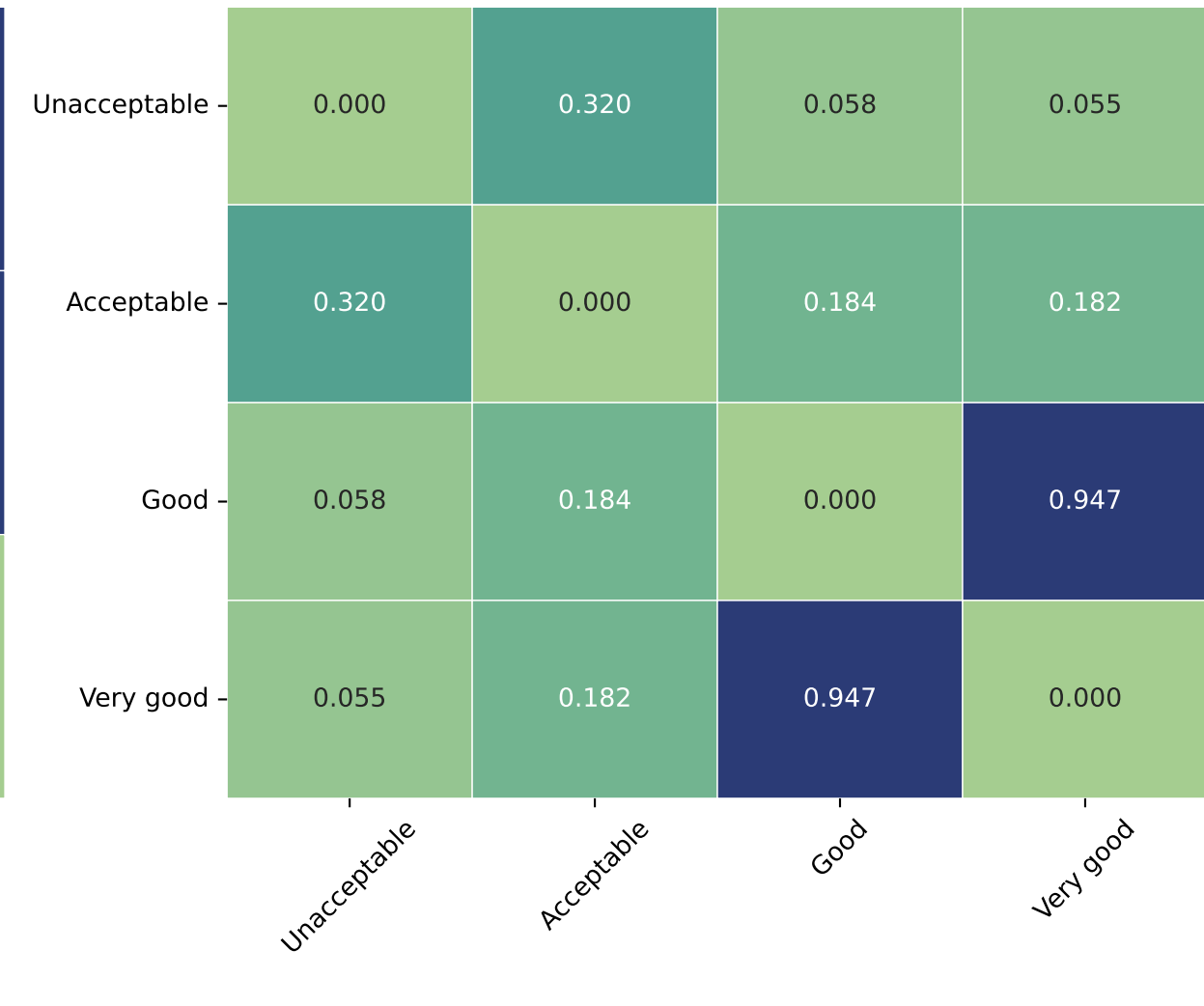
Car Evaluation
