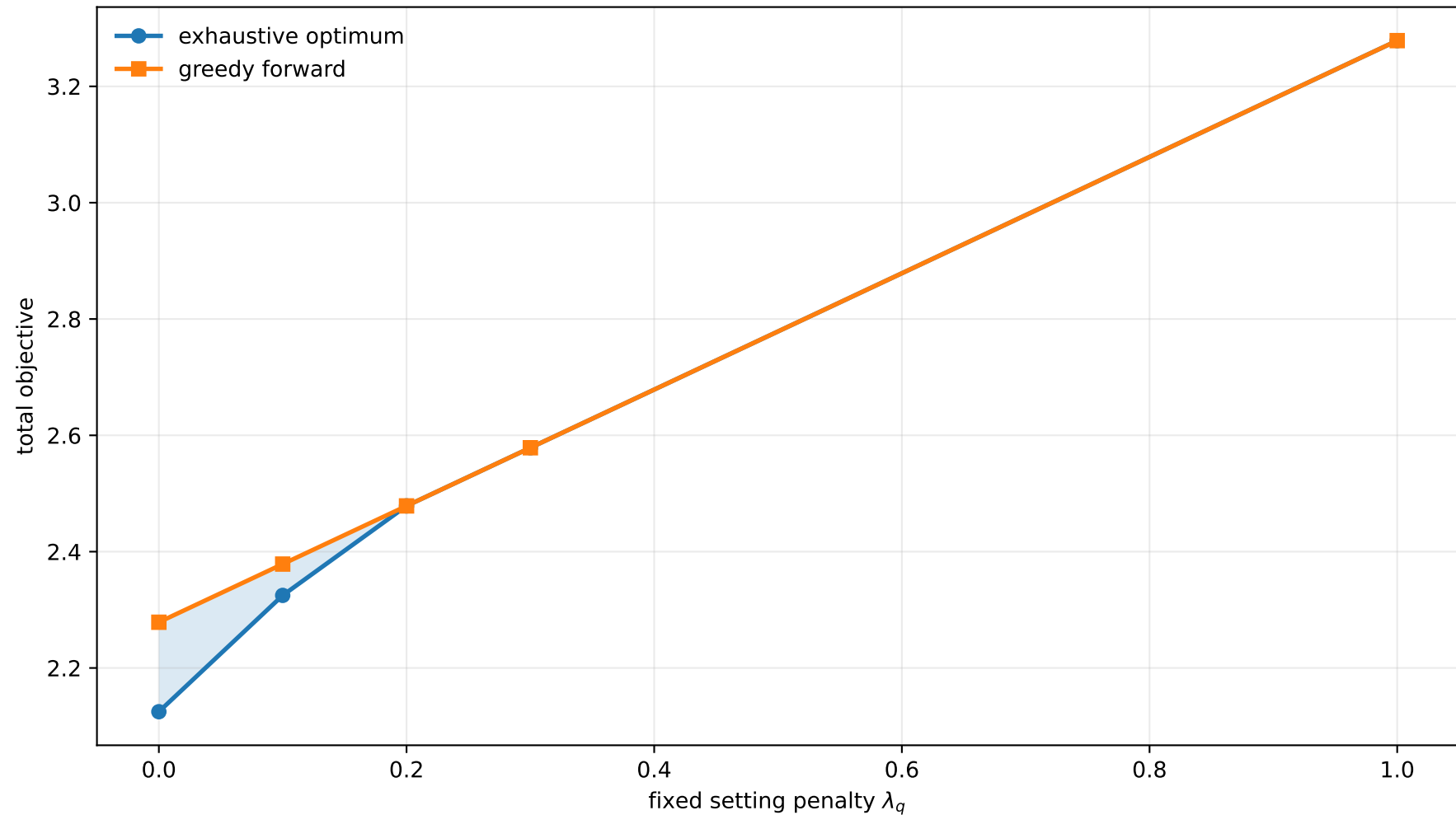
Greedy fixed-setting selection fails in the multi-setting regime
