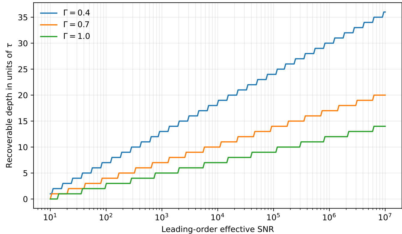
Ideal order-separated depth grows as (\tau/\Gamma)\log(\text{SNR})
