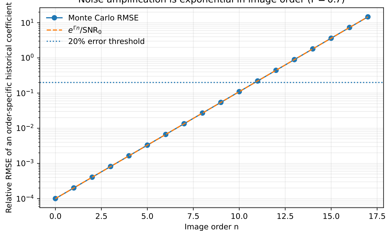
Noise amplification is exponential in image order ( \Gamma = 0.7 )
