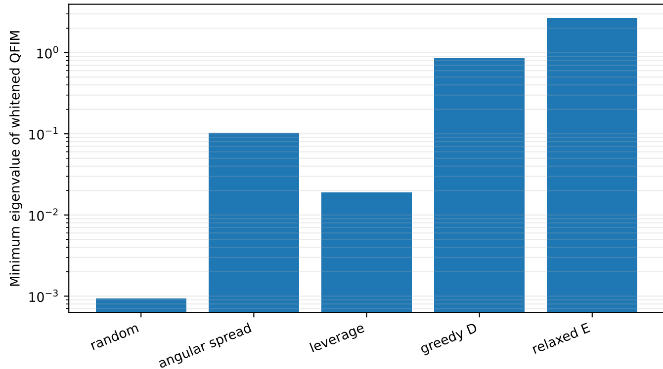
Single synthetic task: design changes the worst visible direction
