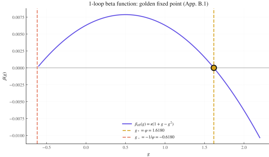
Figure 58: Fig B.1: 1-loop beta function (App.)
