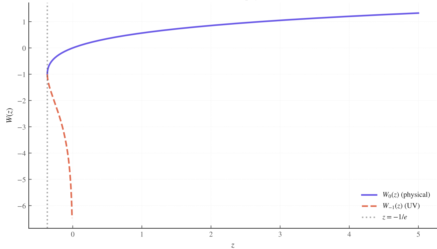
Lambert-W branches (physical vs UV)
