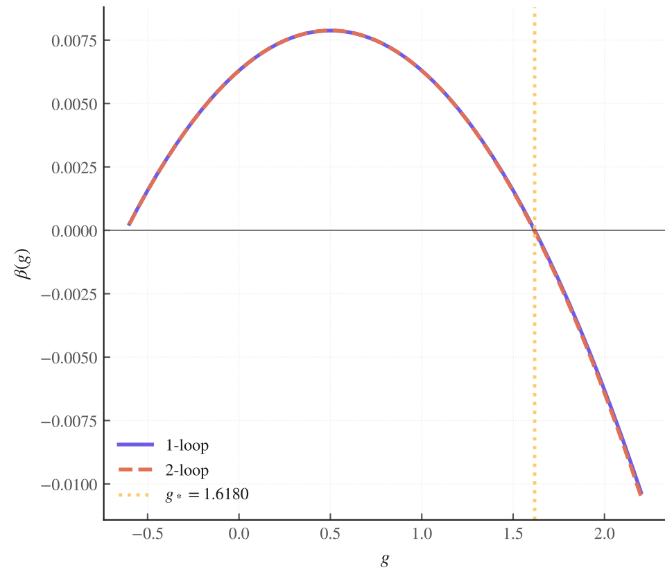
\beta function: 1-loop vs 2-loop
