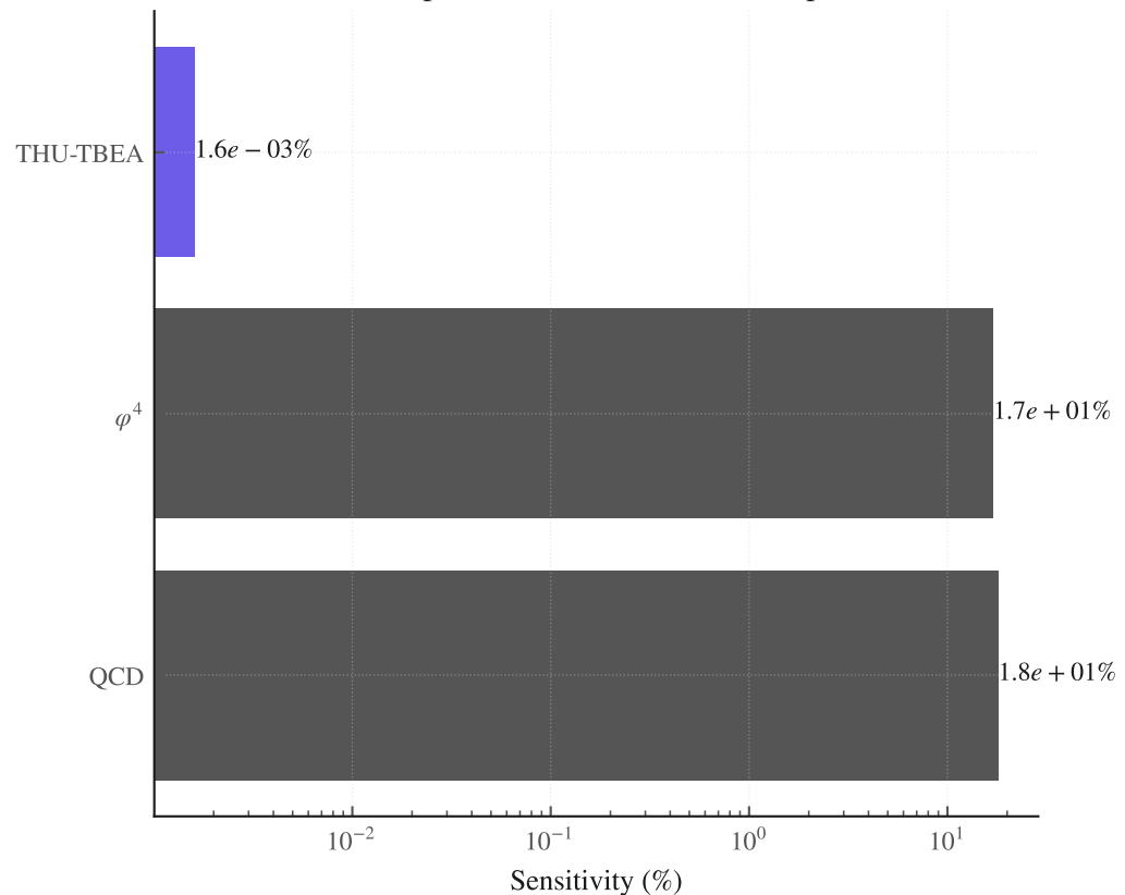
Comparative robustness at 2-loops
