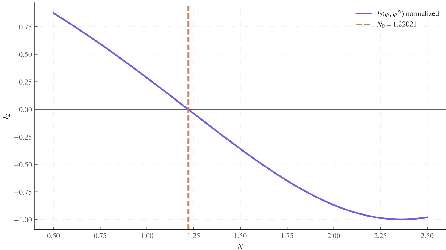
Analytic zero of the scalar vacuum integral
