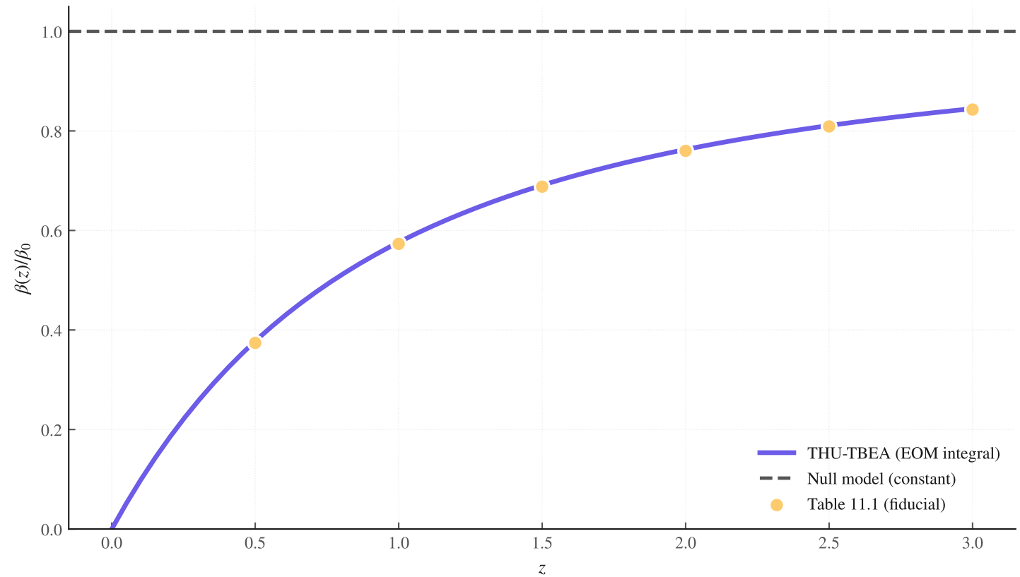
\beta(z) tomography: central falsifiable prediction
