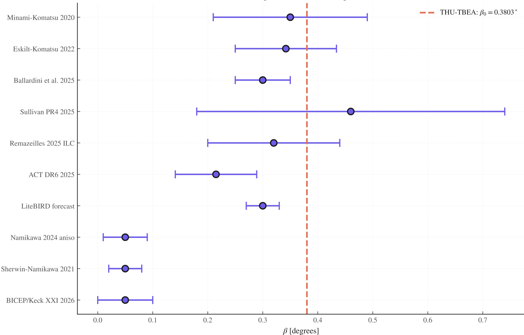
Forest plot: cosmic birefringence
