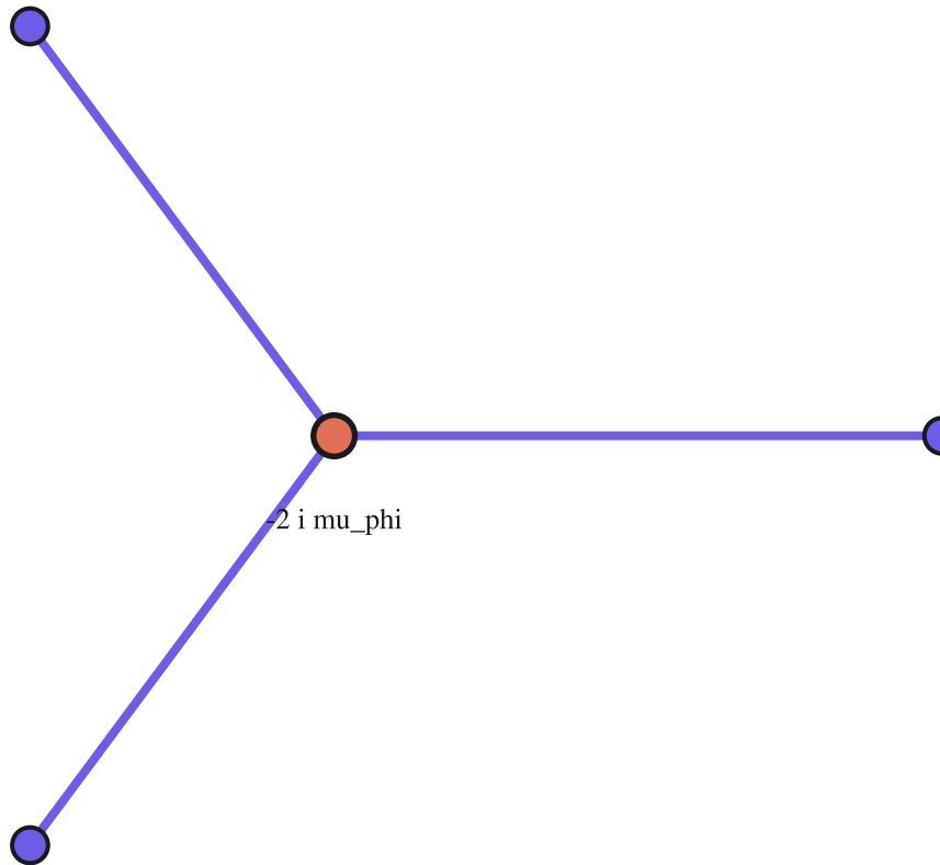
Vertex \Phi\text{-}\tau^2
