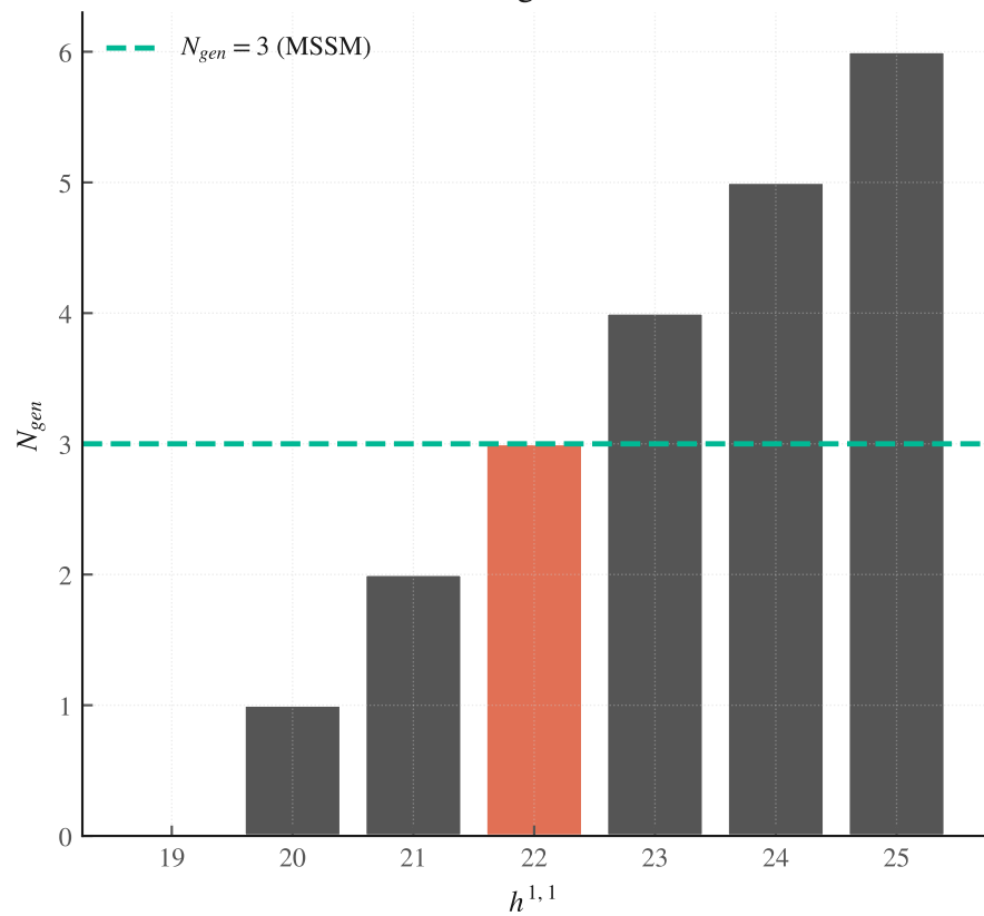
Fermion generations
