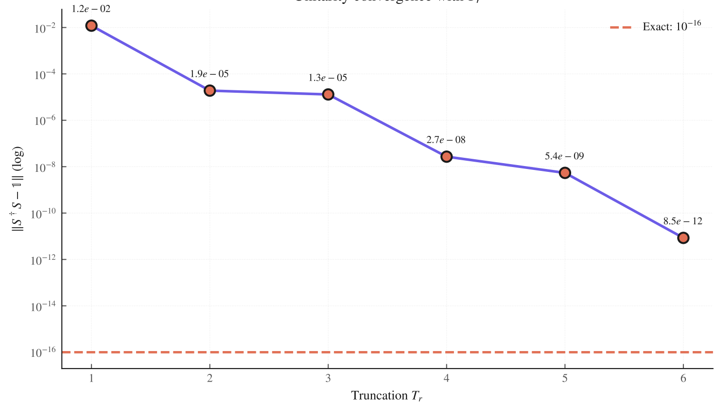
Unitarity convergence with T_r
