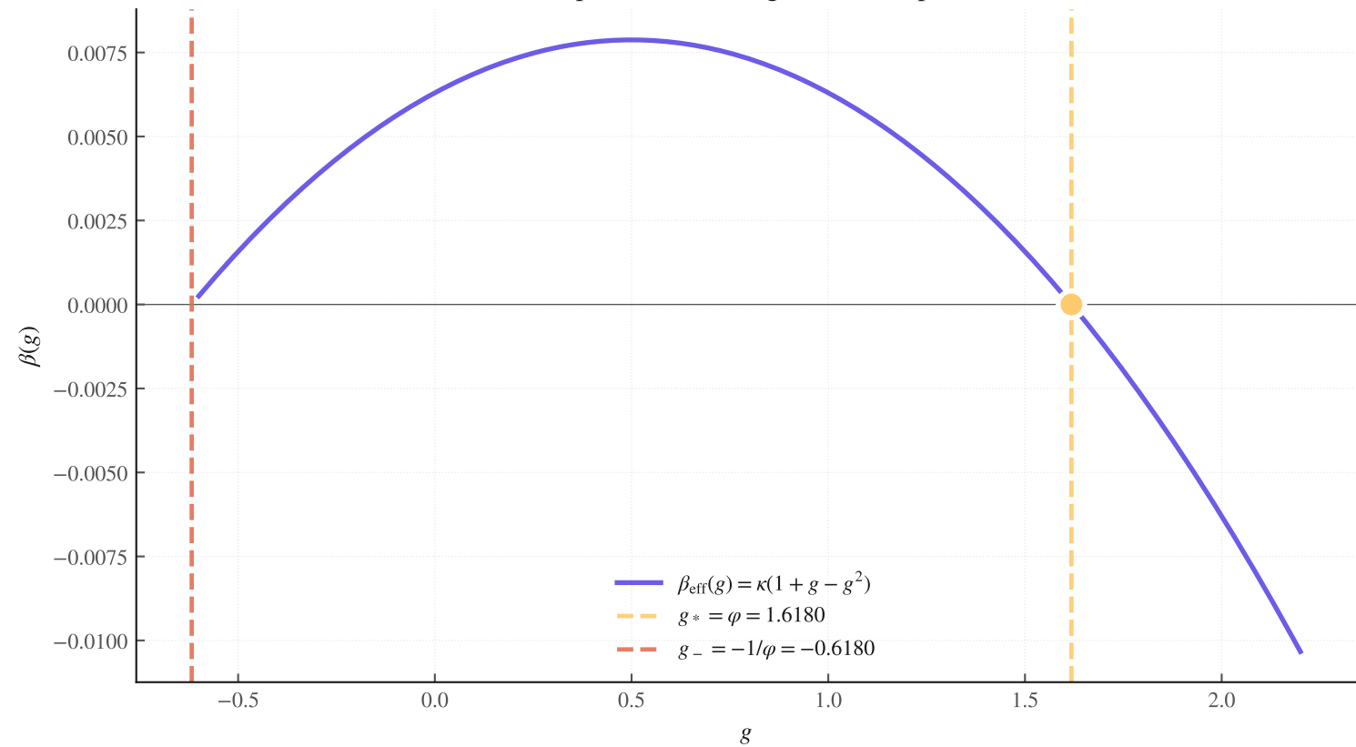
1-loop beta function: golden fixed point
