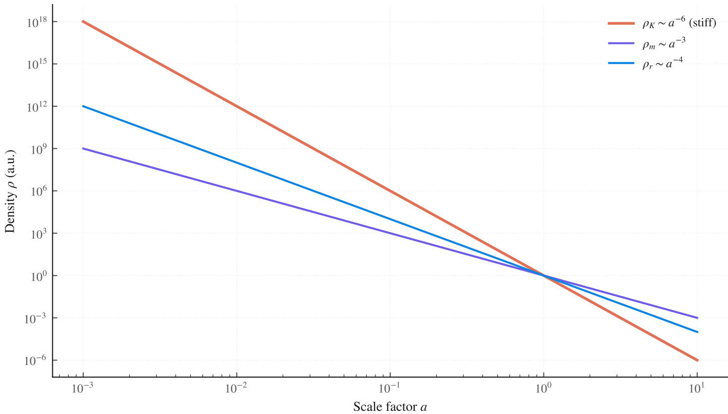
Stiff sector evolution ( w_K = +1 )
