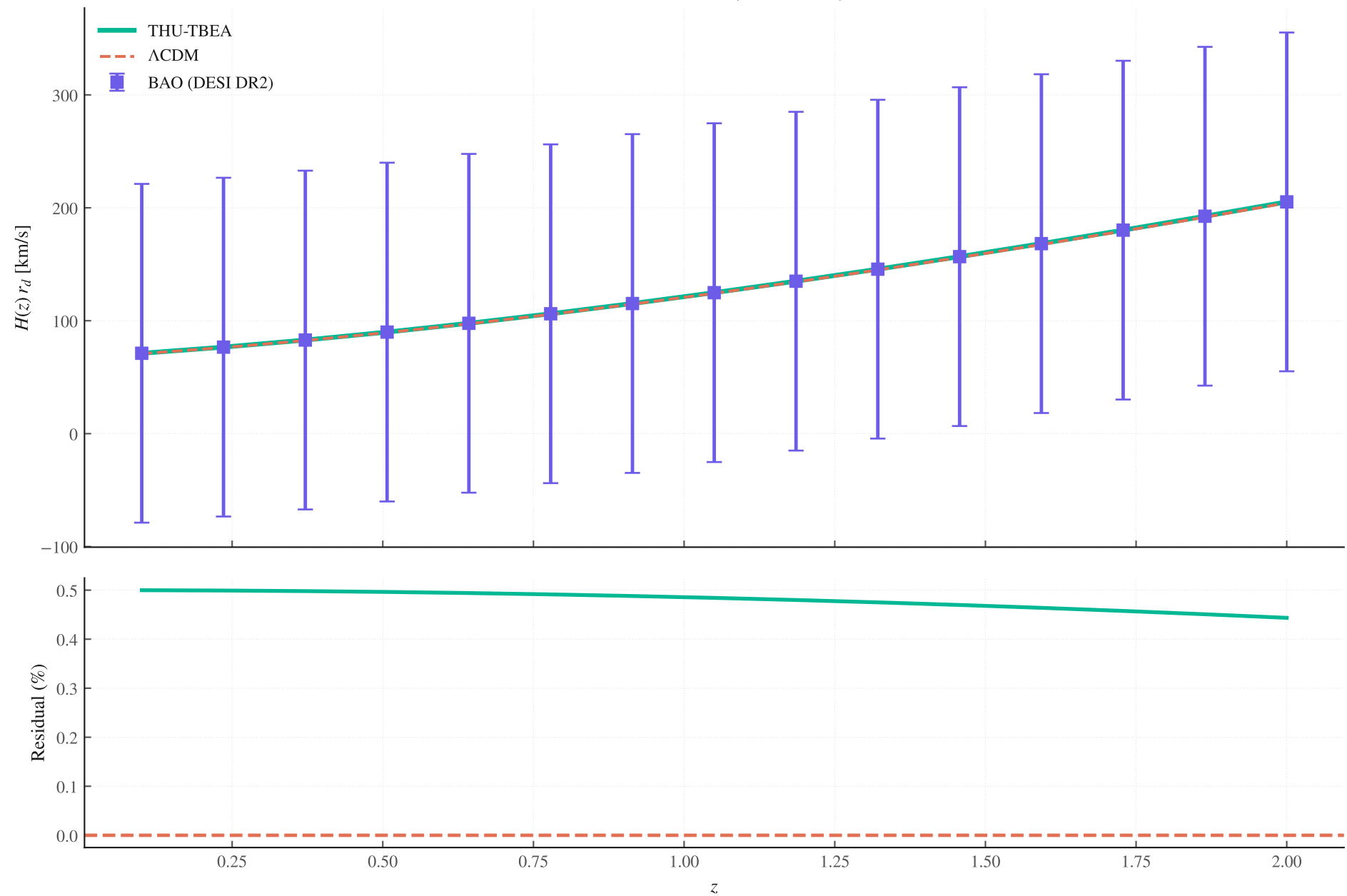
BAO validation (DESI DR2)
