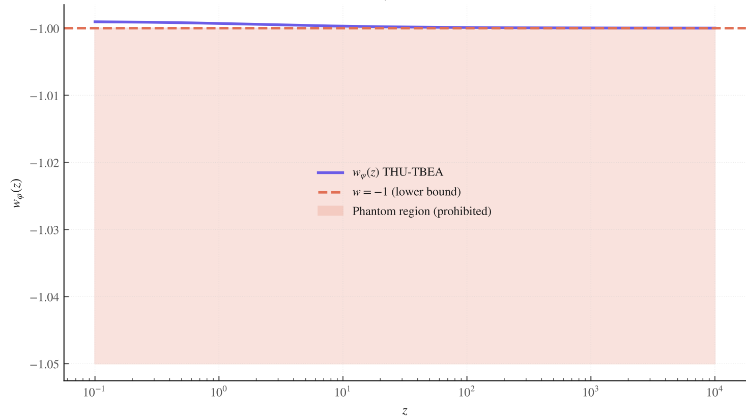
Lower bound w_\phi \geq -1 vs DESI DR2
