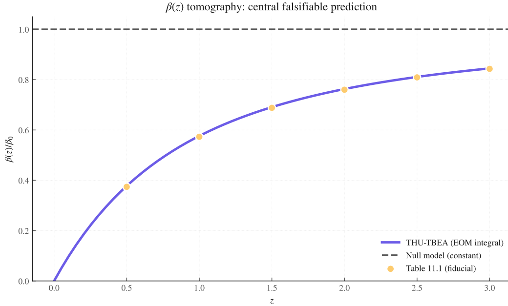
Figure 35: Fig 11.1: tomography
