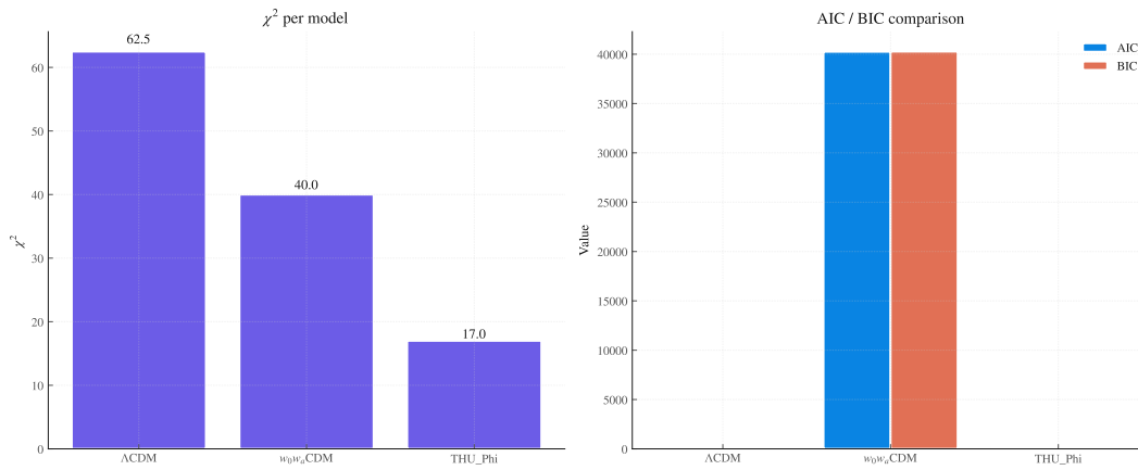
Figure 53: Fig 18.3: AIC/BIC
