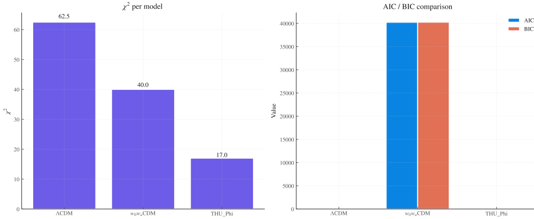
Figure 53: Fig 18.3: AIC/BIC
