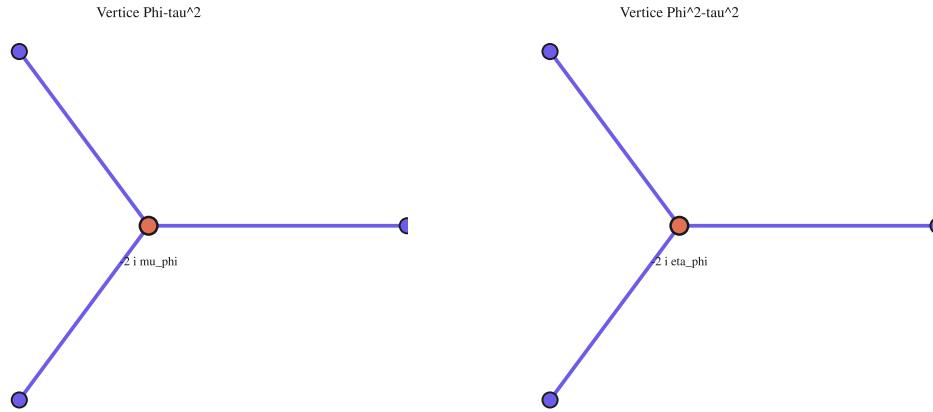
Figure 65: Helical vertices
