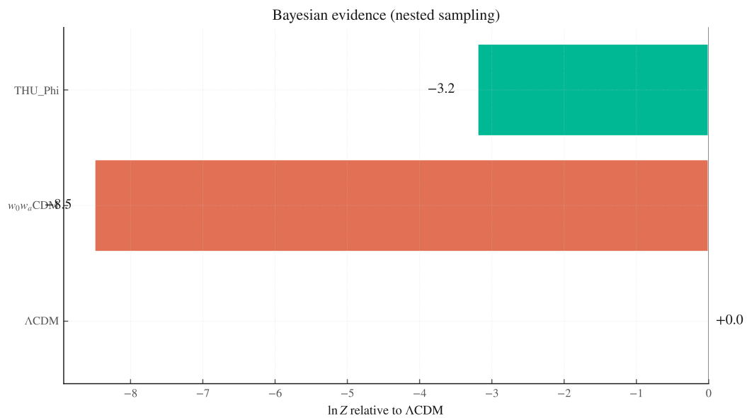
Figure 54: Fig 18.4: Bayesian evidence
