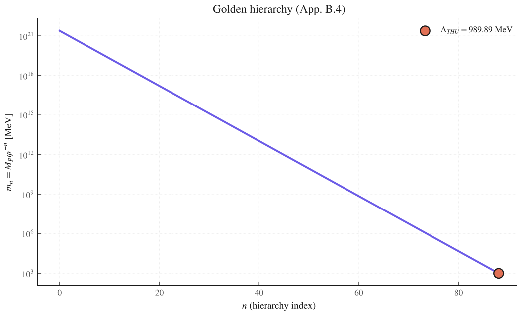
Figure 63: Fig B.4: golden hierarchy
