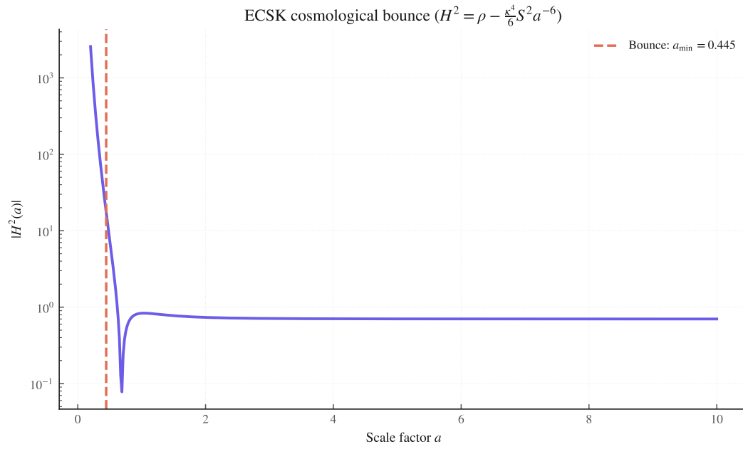
Figure 27: Fig 8.4: ECSK bounce at a_{\min} = 0.445
