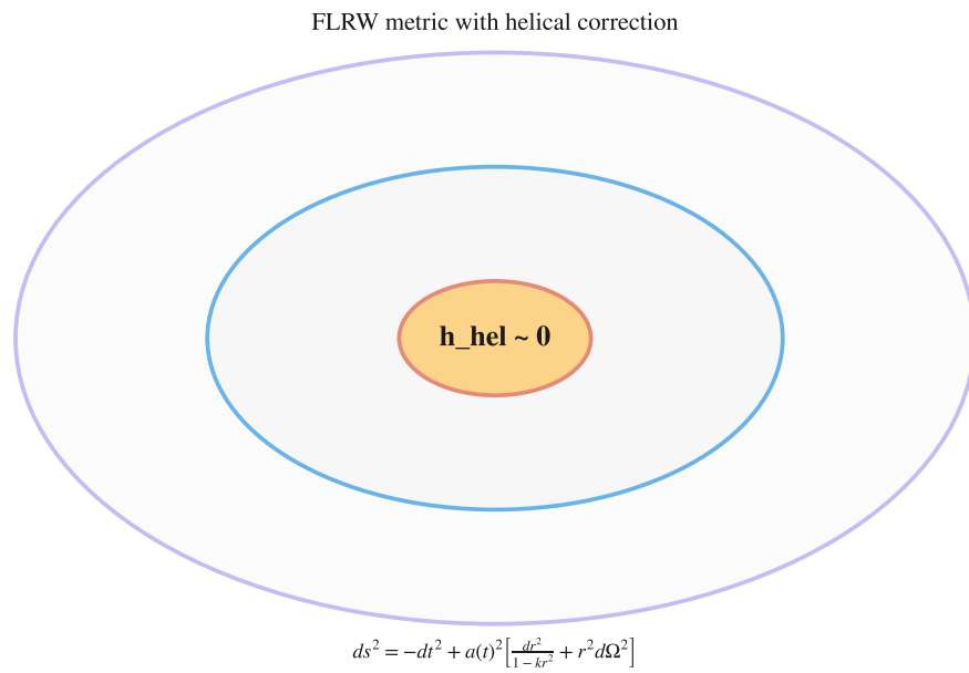
Figure 26: \langle h_{hel} \rangle = 0
