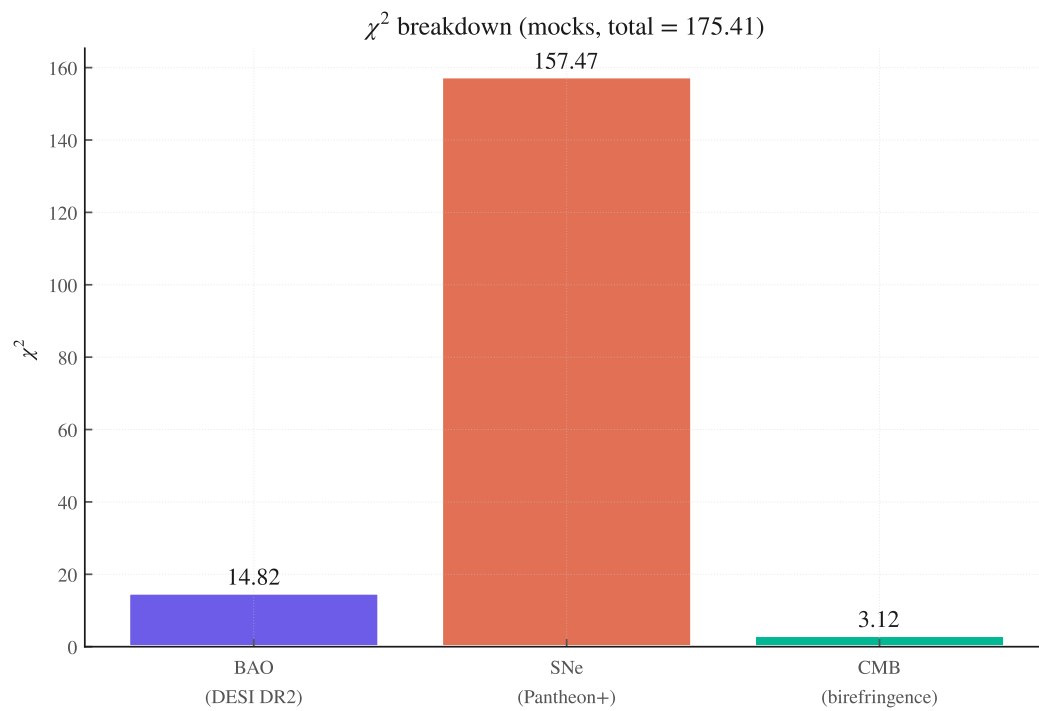
Figure 55: Fig 18.1: \chi^2 breakdown
