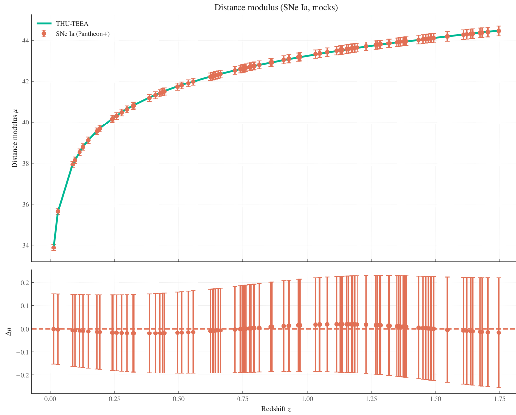
Figure 44: Fig 13.3: Pantheon+ mocks (helical residual)
