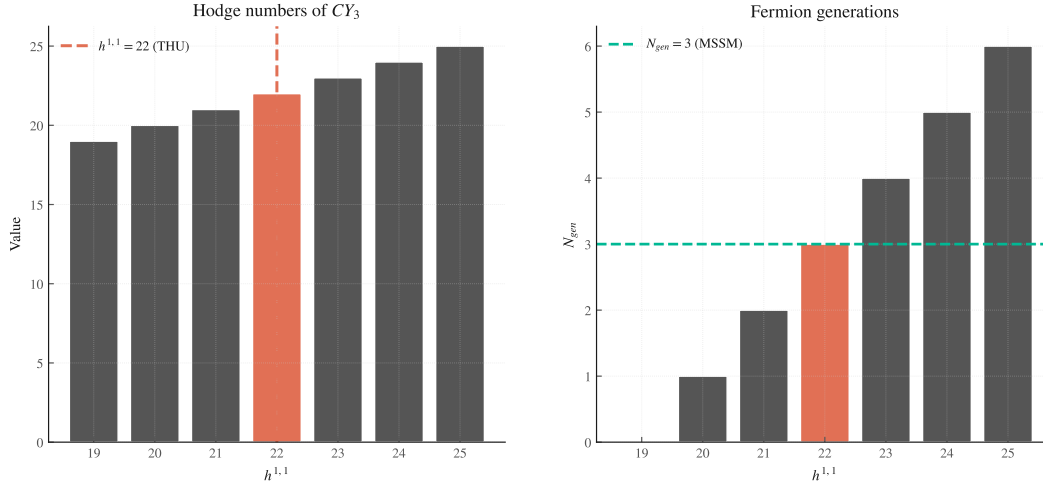
Figure 7: Fig 3.7: h^{1,1}=22 and N_{gen}
