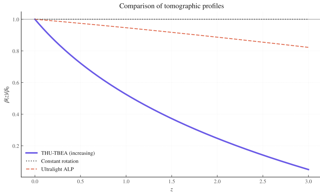
Figure 36: Fig 11.2: profile comparison
