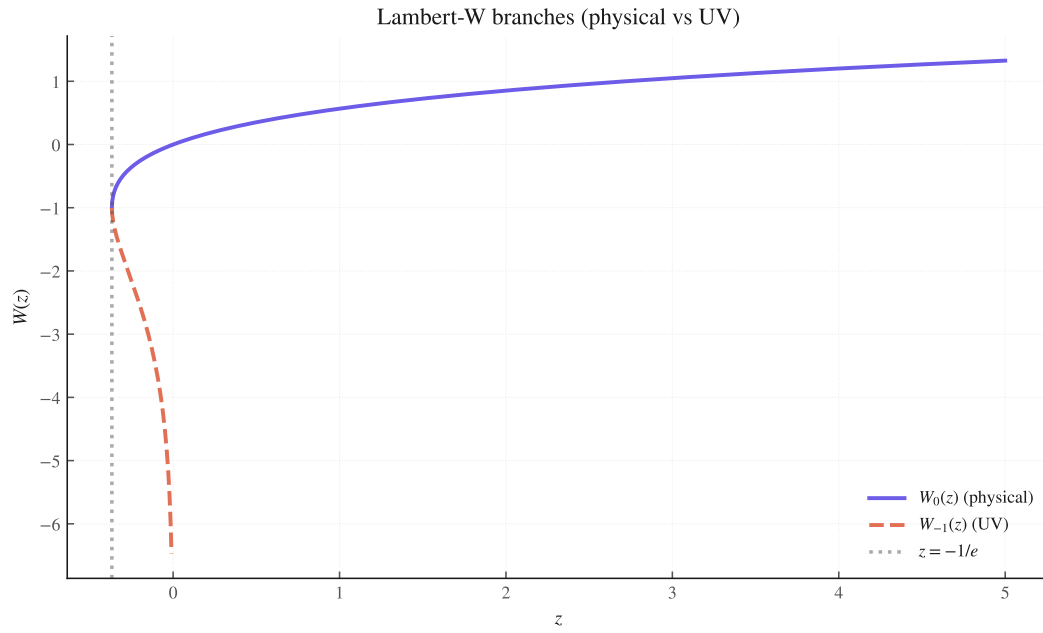
Figure 9: Fig 4.2: Lambert-W branches
