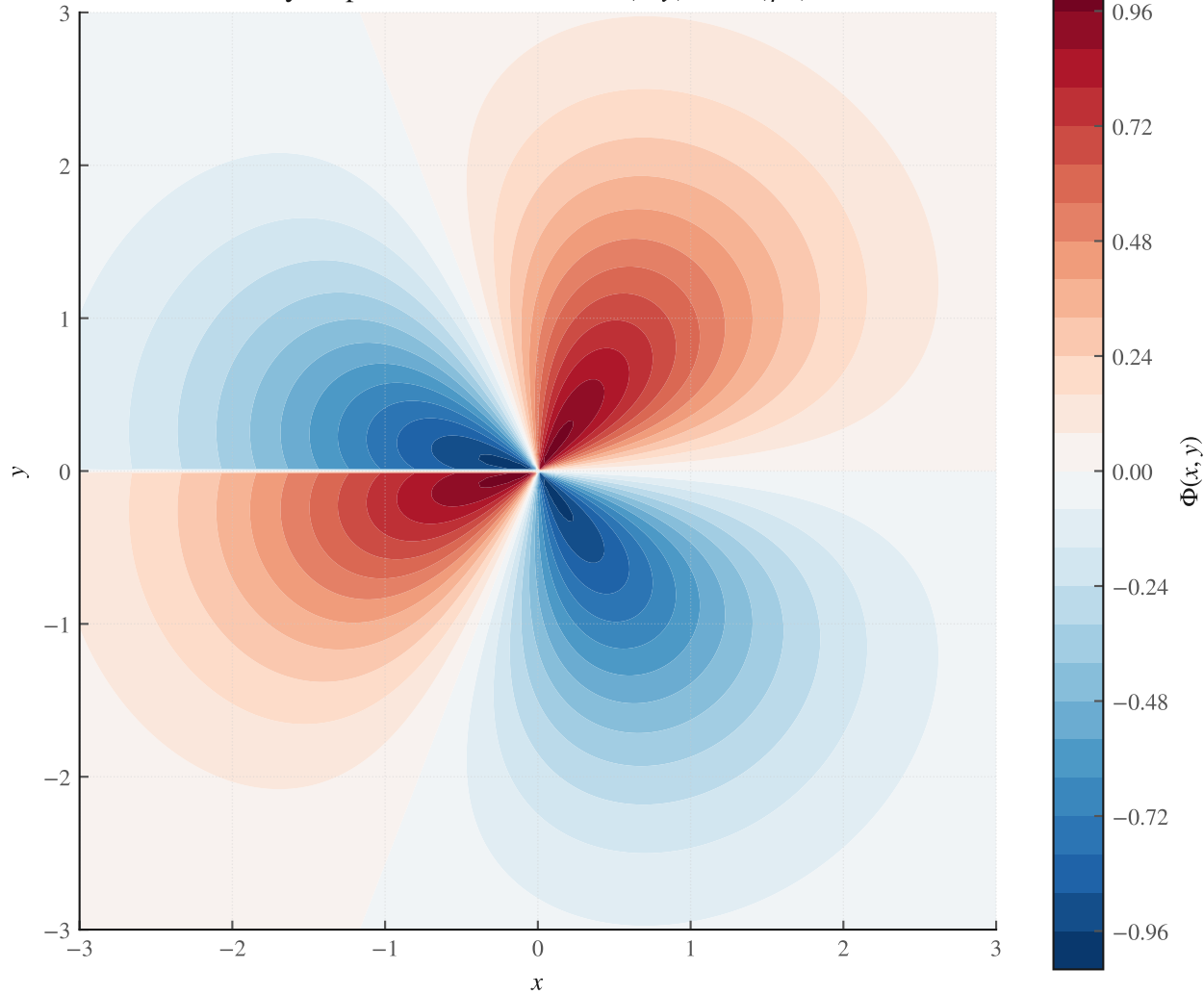
Intensity map of the helical field \Phi(x, y) = \sin(\varphi\theta)e^{-R^2/4}
