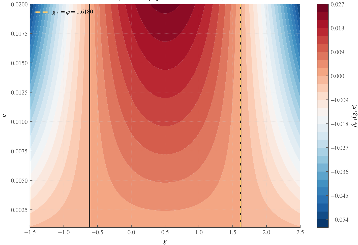
RG phase map ( \beta = 0 curve in white)
