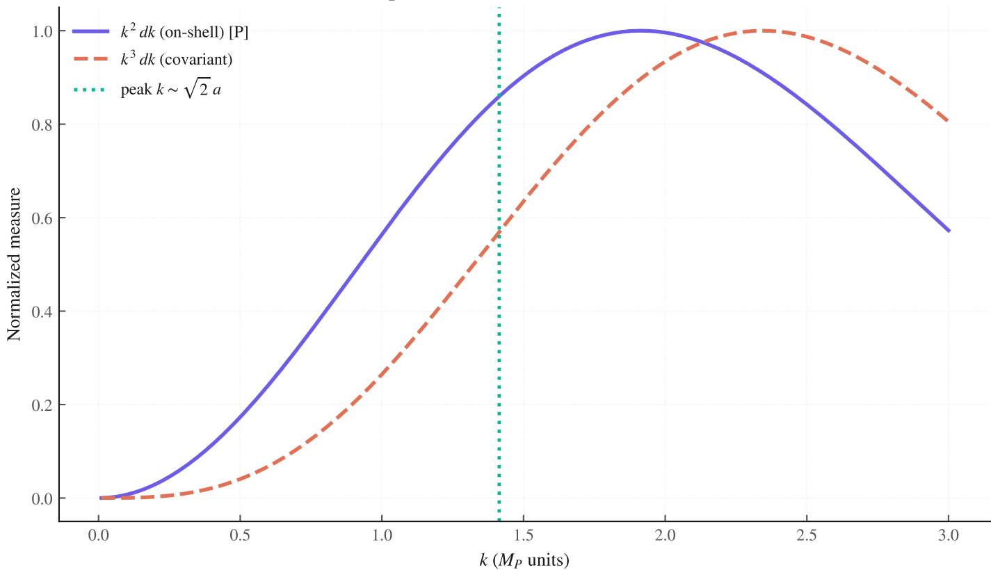
Spectral measures: k^2 dk vs k^3 dk
