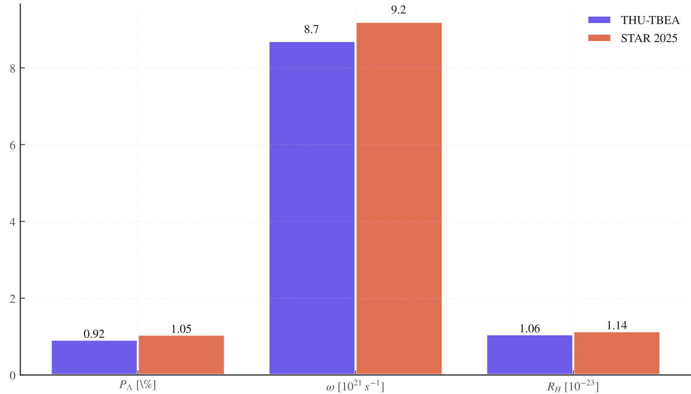
THU prediction vs STAR 2025 (within 1\sigma )
