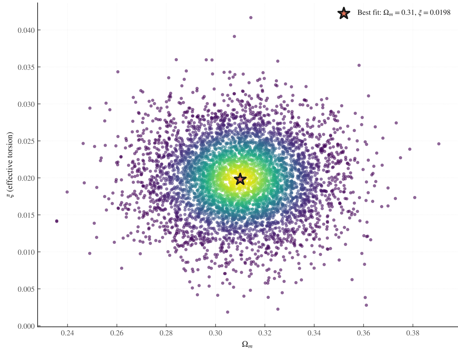
Joint confidence contours (BAO + SNe + CMB)
