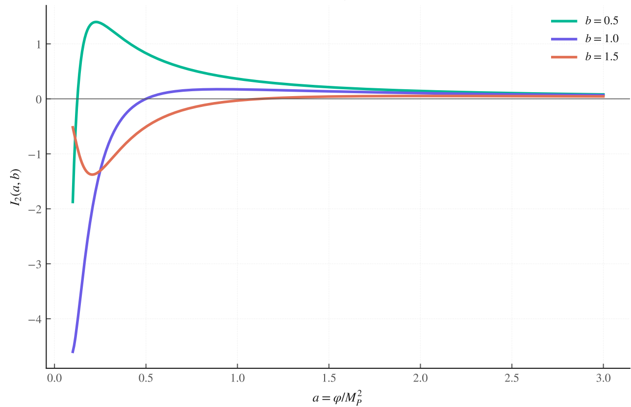
Vacuum integral I_2(a, b)
