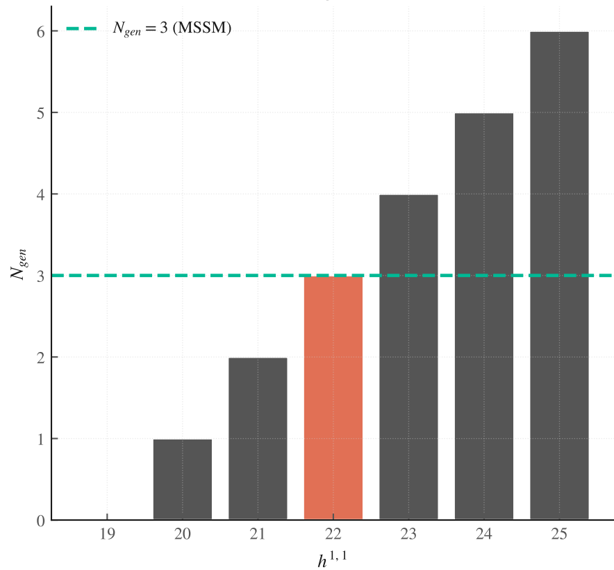
Fermion generations
