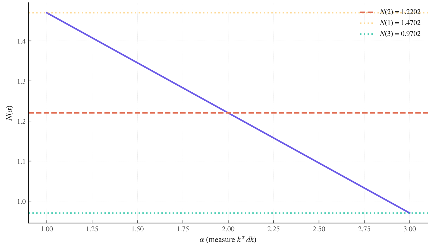
Sensitivity to the spectral measure
