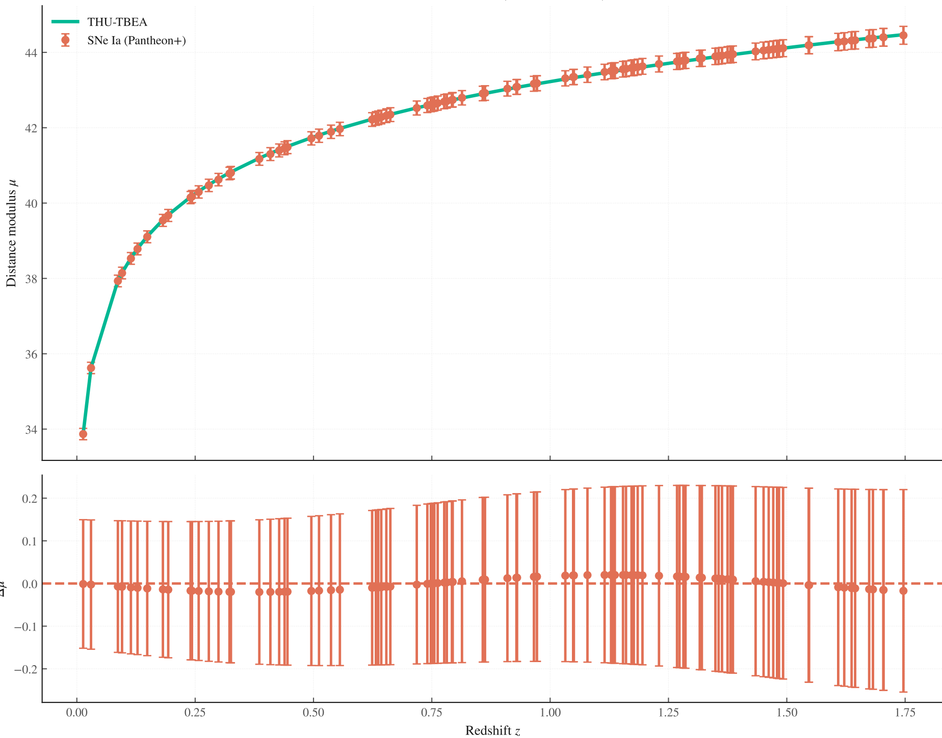
Distance modulus (SNe Ia, mocks)
