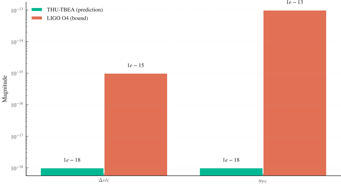
A-5: prediction vs LIGO O4 bound
