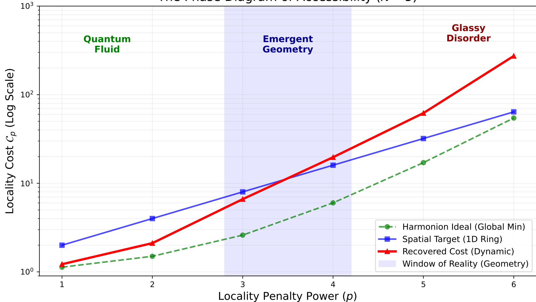
The Phase Diagram of Accessibility ( N = 5 )
