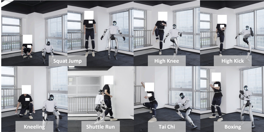
Fig. 7. Whole-body motion capability. The same Unitree G1 policy tracks live whole-body commands for squat jumps, high knees, high kicks, kneeling, shuttle runs, Tai Chi, and boxing.
