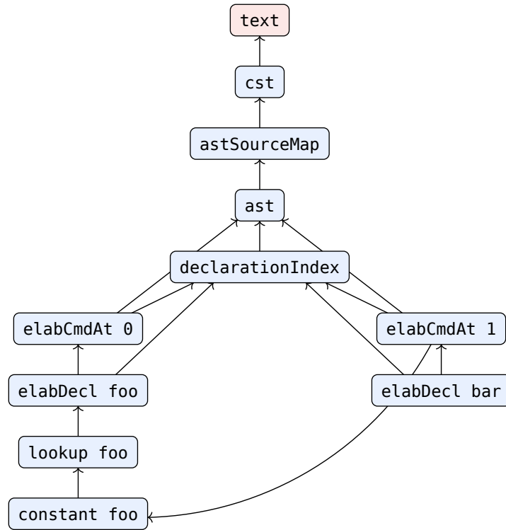
Figure 4: Query dependency graph for a file with two definitions. Arrows point from a query to its dependencies. The text node (red) is the input. Elaborating bar depends on constant foo, which depends on elabDecl foo. Editing foo’s body invalidates elabCmdAt 0, elabDecl foo, lookup foo, and constant foo; if the resulting Constant hashes the same (e.g. the type is unchanged), elabDecl bar is not recomputed.
