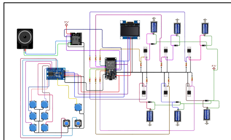
System Schematic
