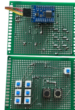
Input Circuit
