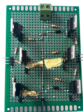
Solenoid Driver Circuit
