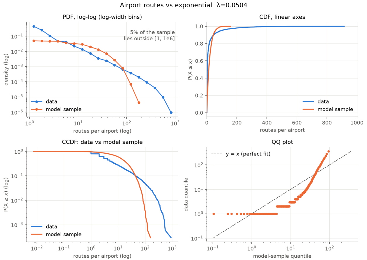
Figure 3: Airport routes vs. samples from the fitted exponential.
