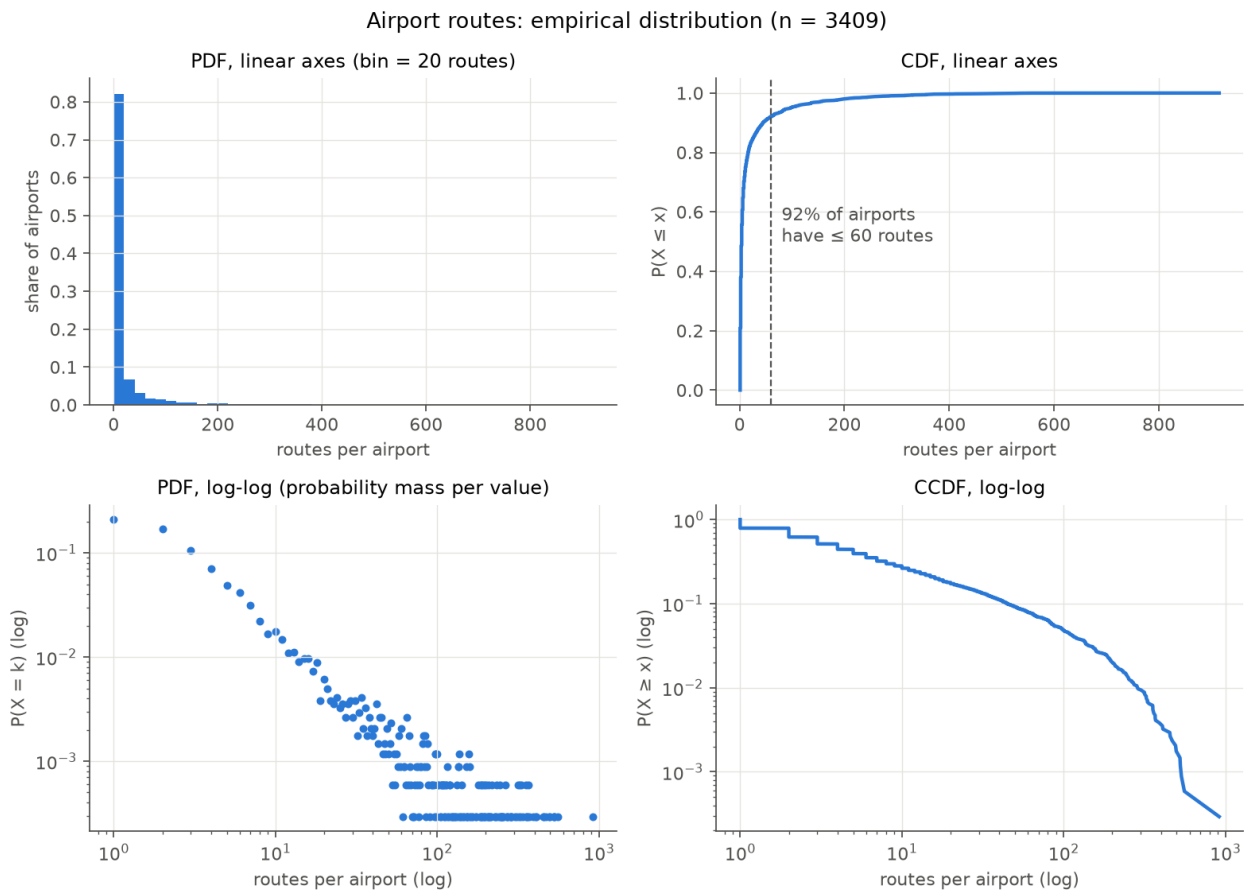
Figure 1: Airport routes: PDF and CDF on linear axes (top), PDF and CCDF on log-log axes (bottom).
