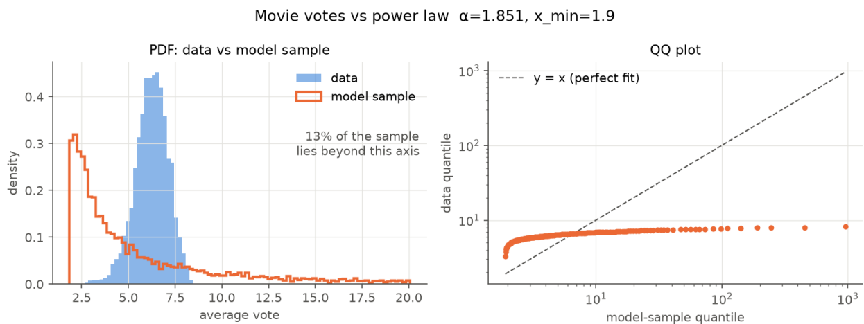
Figure 7: Movie votes vs. samples from the fitted power law.
