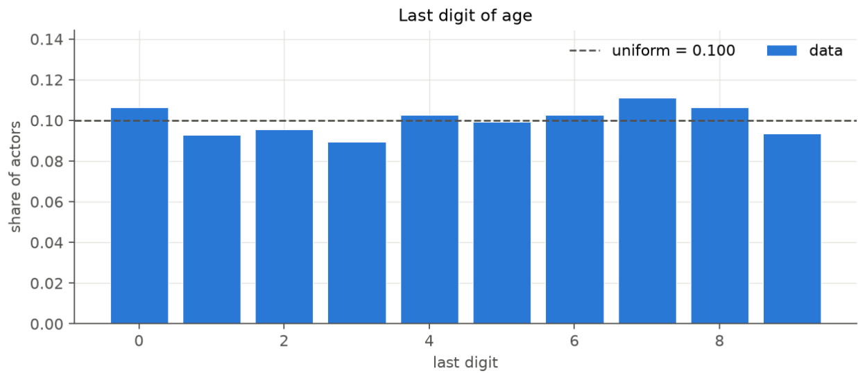
Figure 13: Distribution of the last digit of age.
