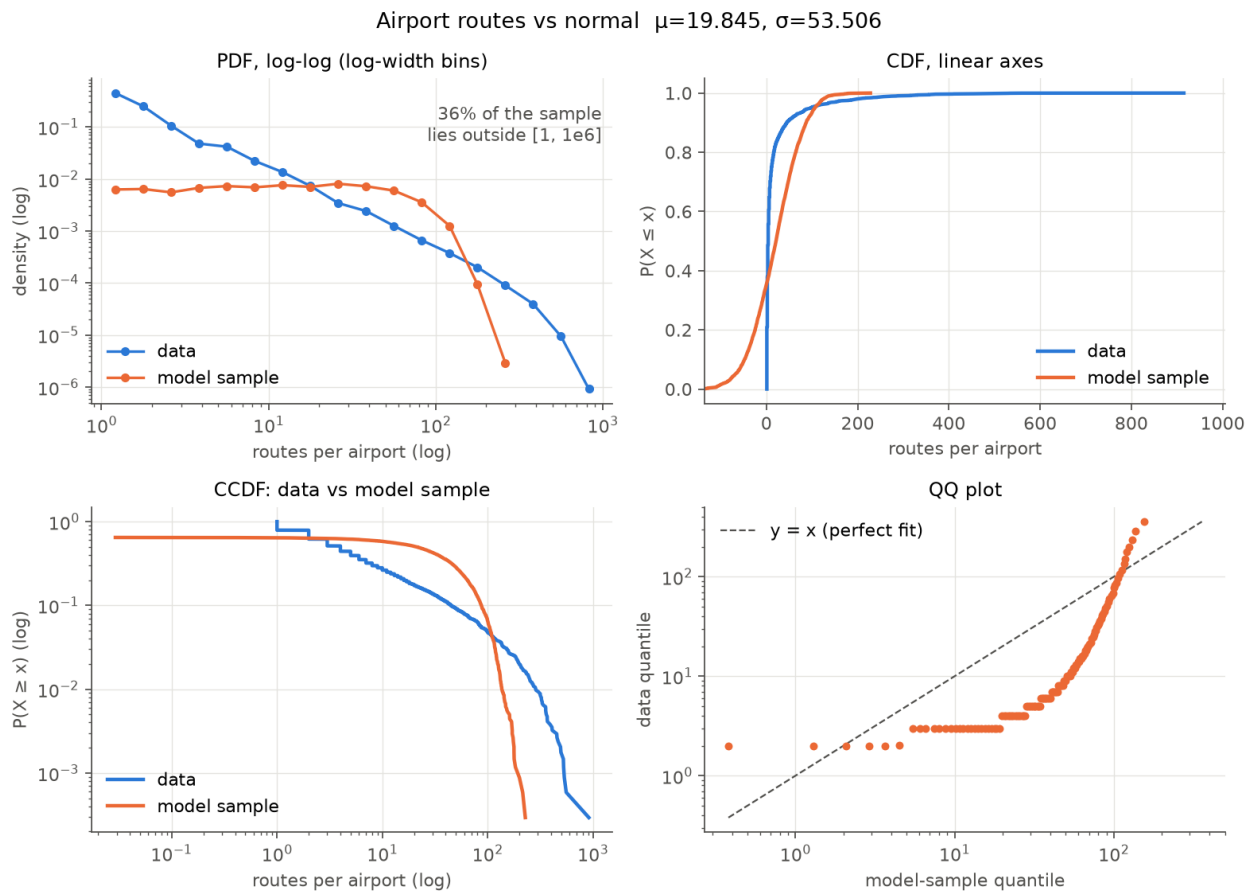
Figure 5: Airport routes vs. samples from the fitted normal.
