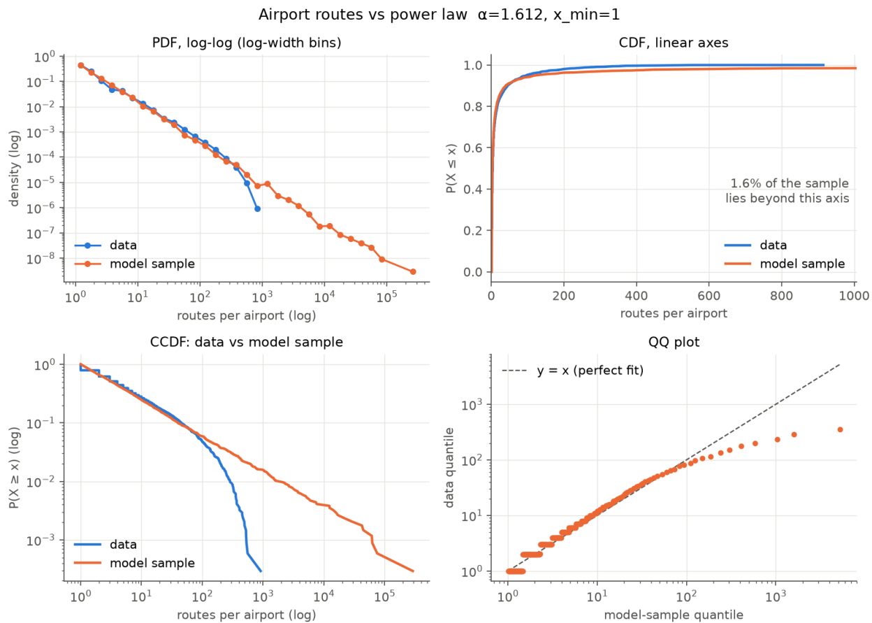
Figure 2: Airport routes vs. samples from the fitted power law.
