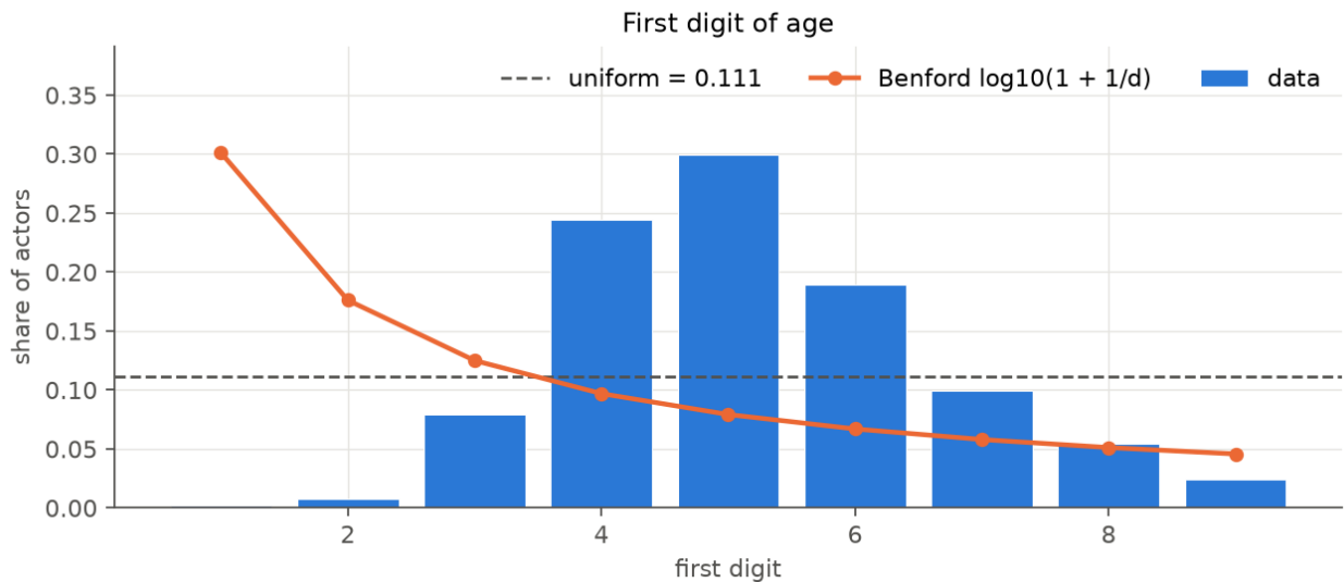
Figure 12: Distribution of the first digit of age.
