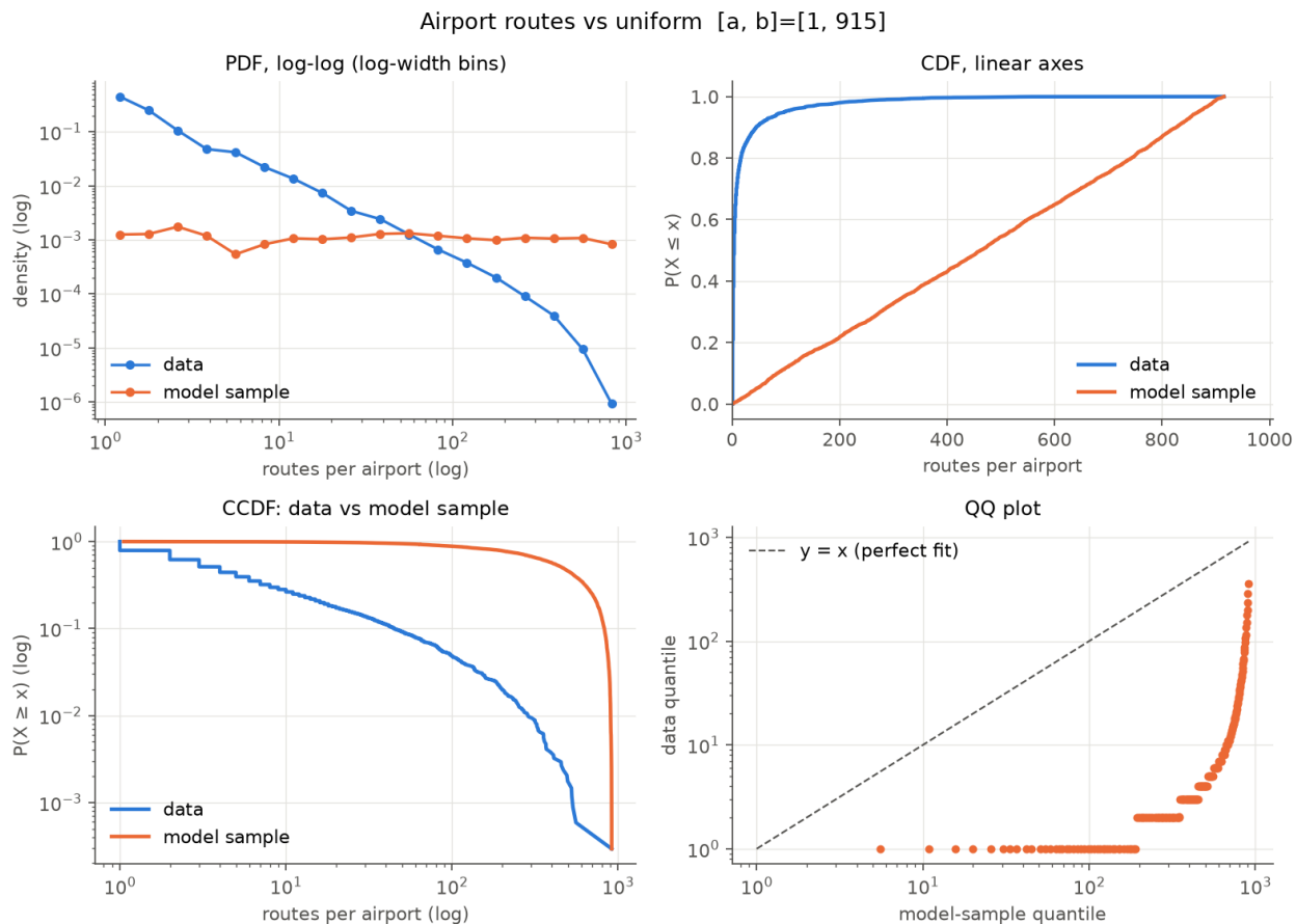
Figure 4: Airport routes vs. samples from the fitted uniform.
