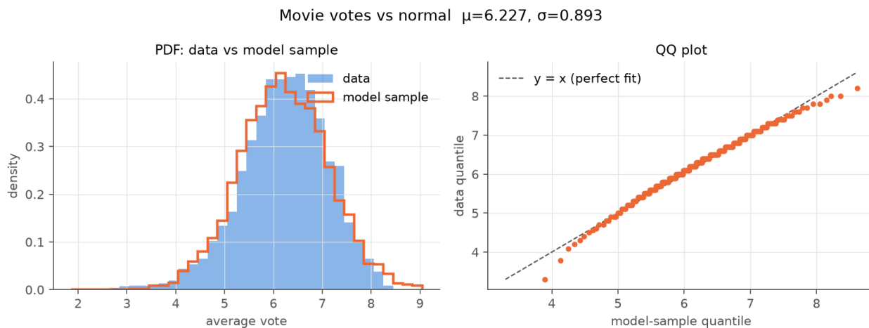
Figure 10: Movie votes vs. samples from the fitted normal.
