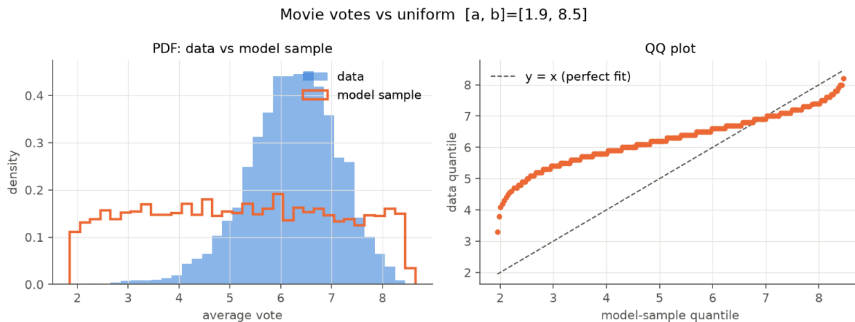
Figure 9: Movie votes vs. samples from the fitted uniform.
