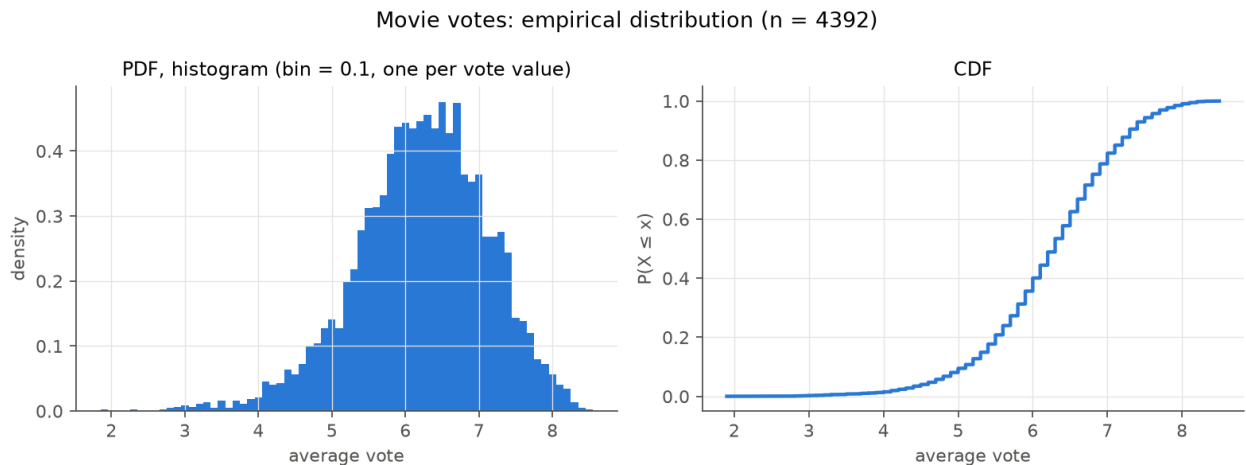
Figure 6: Movie votes: empirical PDF (histogram) and CDF.
