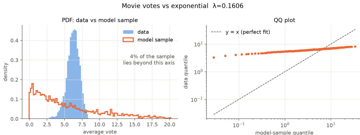
Figure 8: Movie votes vs. samples from the fitted exponential.
