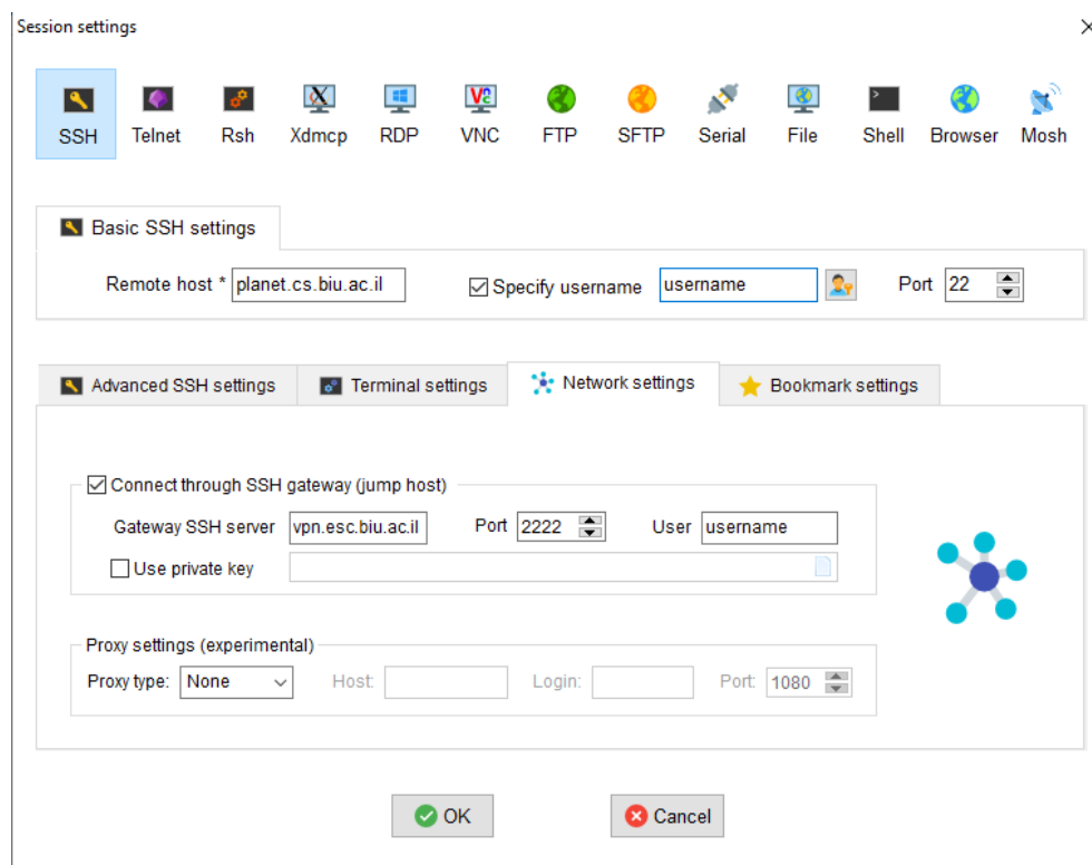
Figure 4: MobaXterm SSH and jump-host settings.
