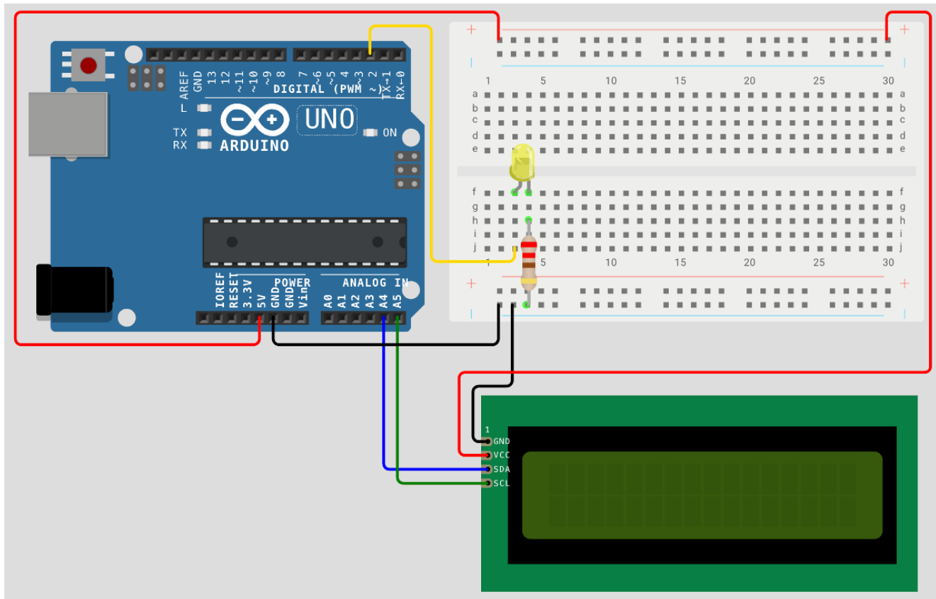
Figure 1: Exercise 0 circuit. Follow the diagram exactly.
