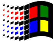
Windows 3.1
