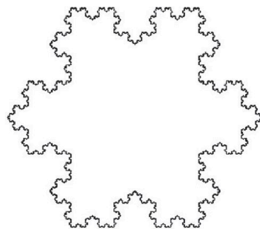
Koch Snowflake
