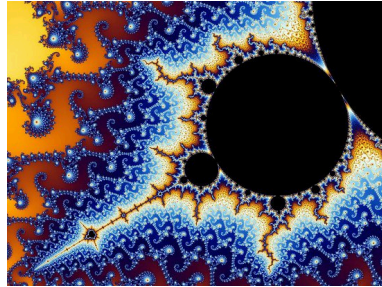
Mandelbrot Set
