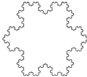
Koch Snowflake
