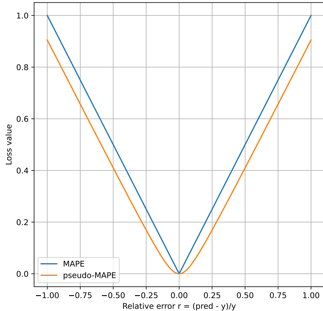
Loss functions
