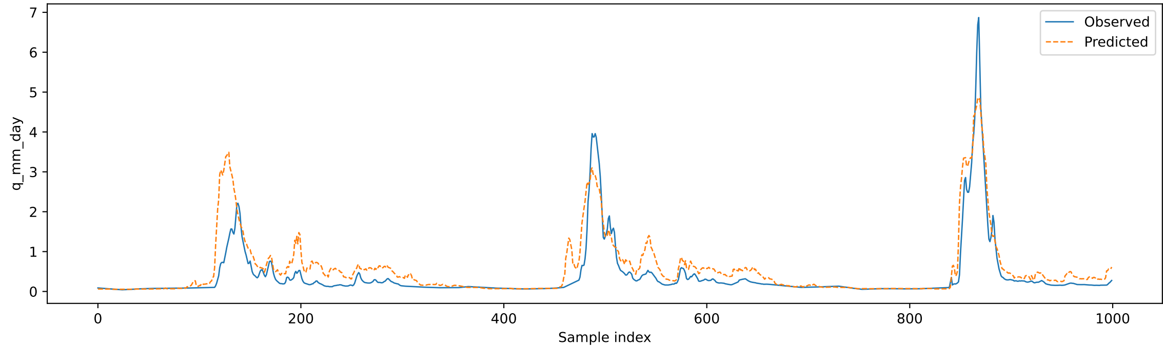
Gradinet Boosting Preds (Gauge 8249)
