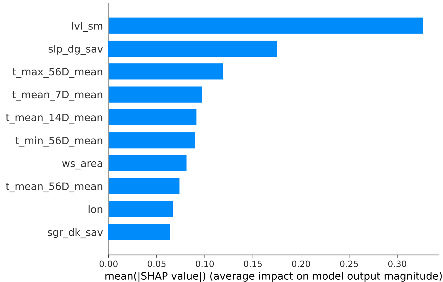
RF SHAPS (Cluster 0)
