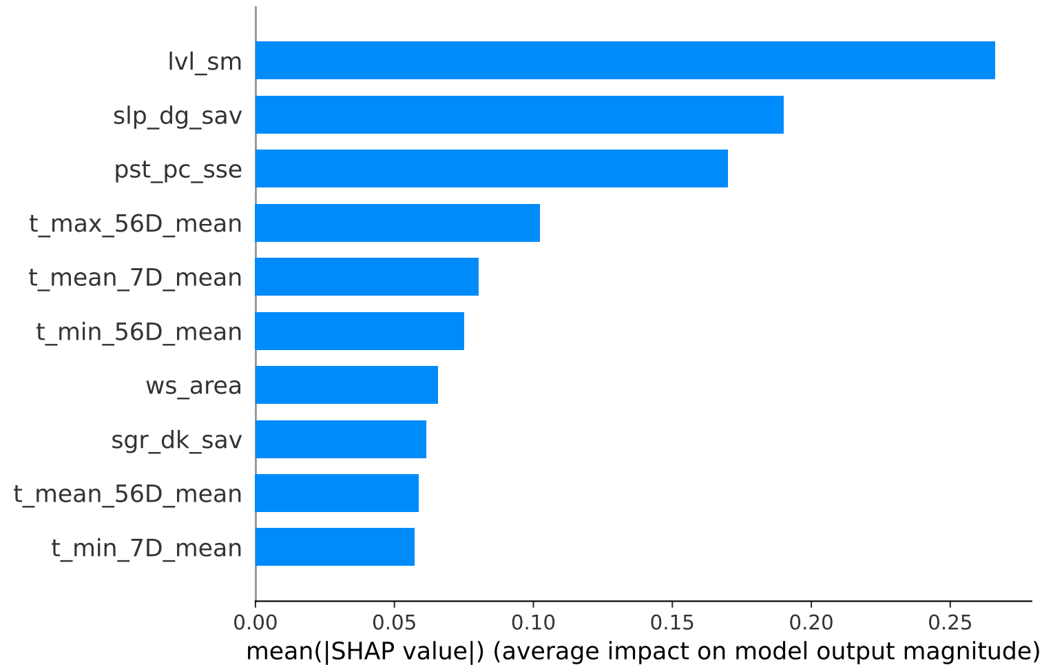
RF SHAPS (Cluster 1)
