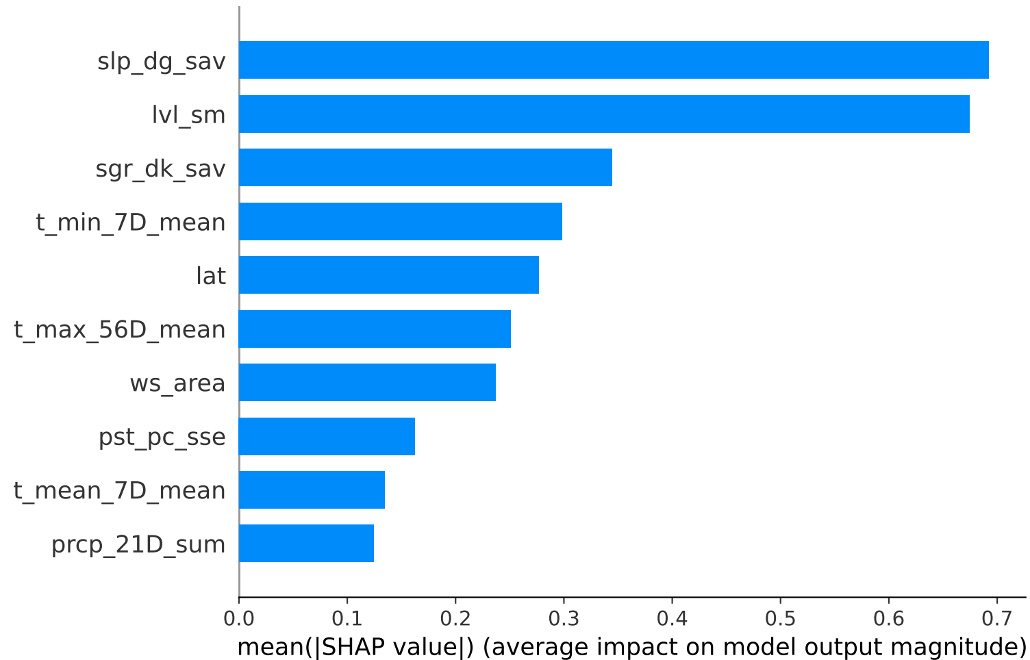
RF SHAPS (Cluster 4)
