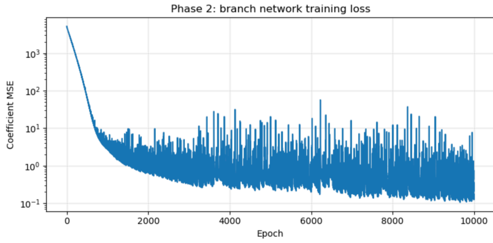
Figure 6: Phase 2 MSE training curve for POD-DeepONet on 1D Burgers' ( \nu=1.0 ).
