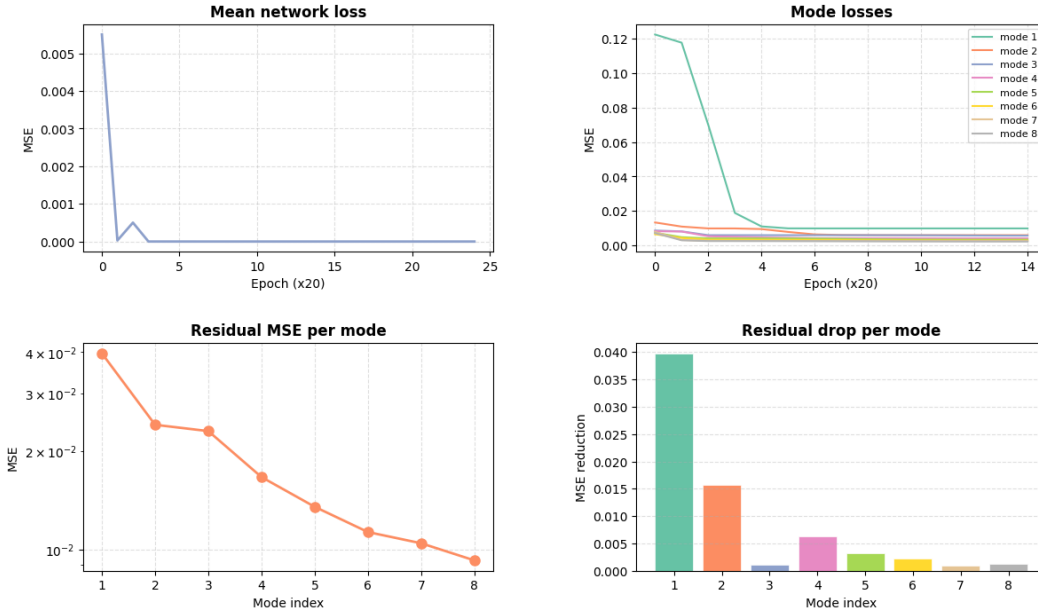
Figure 2: Fourier NeuralPOD training dynamics on 1D Burgers' ( \nu=1.0 ): residual MSE per greedily added mode.
