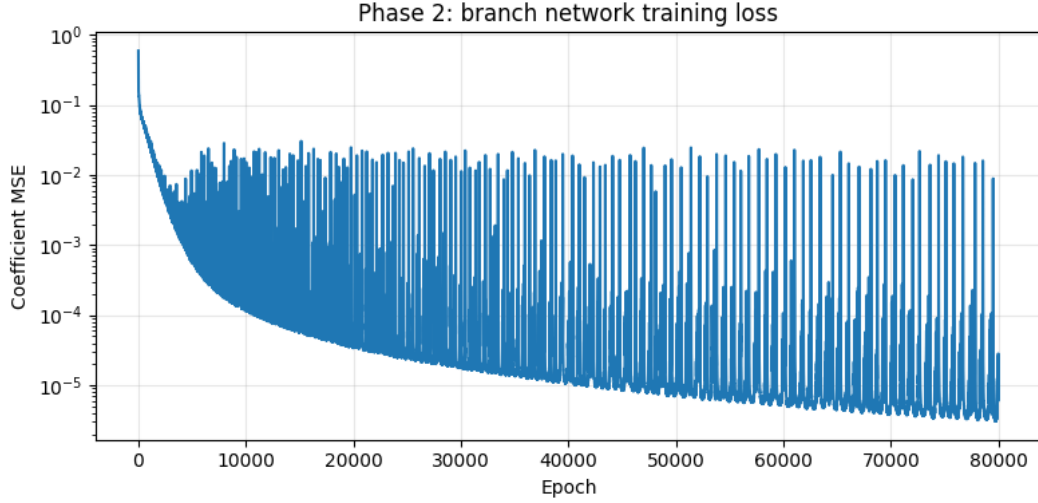
Figure 6: Phase 2 MSE training curve for NeuralPOD-DeepONet on 1D Burgers' ( \nu=1.0 ).
