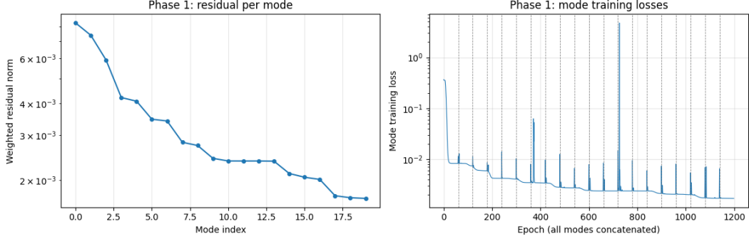
Figure 4: Fourier NeuralPOD basis on 1D Burgers' ( \nu=1.0 ): weighted residual norm as a function of greedy mode count.
