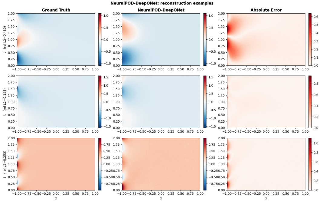
Figure 8: NeuralPOD-DeepONet: representative reconstructions on 1D Burgers' ( \nu=1.0 ). Layout as in Figure 7.
