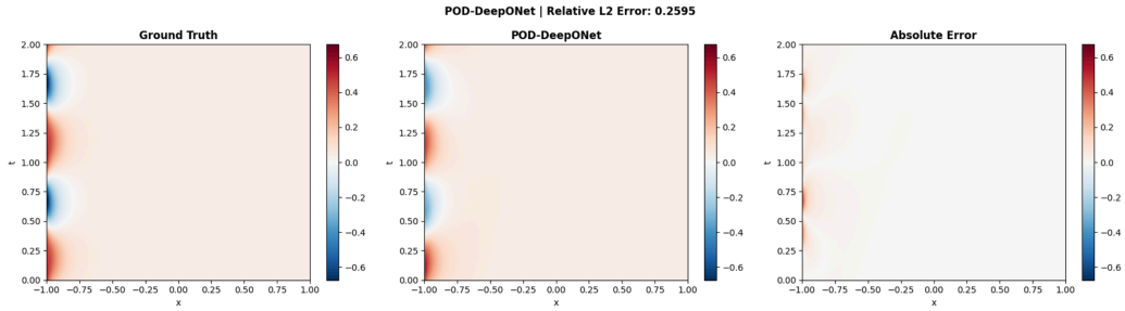
Figure 7: POD-DeepONet: representative reconstructions on 1D Burgers' ( \nu=1.0 ). Each row shows one test snapshot: ground truth ( left ), prediction ( centre ), and point-wise absolute error ( right ).
