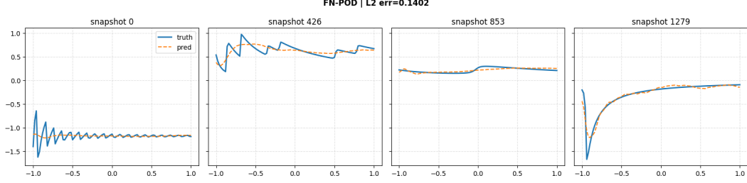
Figure 3: Learned Fourier NeuralPOD basis functions and representative reconstructions on 1D Burgers' ( \nu=1.0 ).
